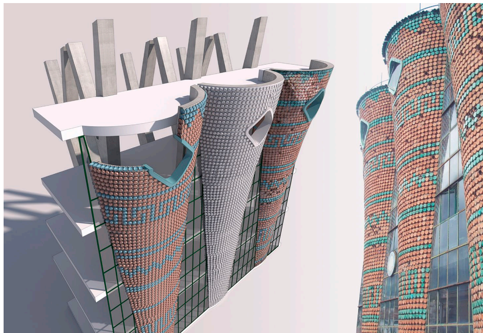
From laser scanner acquisition to HBim model from Solimene Factory (Vietri sul Mare Italy) [A.Rossi et.al. 2024.Between Memory and Reason: The Brick Wall, TEMA.Vol. 10, No. 1 (2024) Fig. 7 Autore Santiago Lillo]
