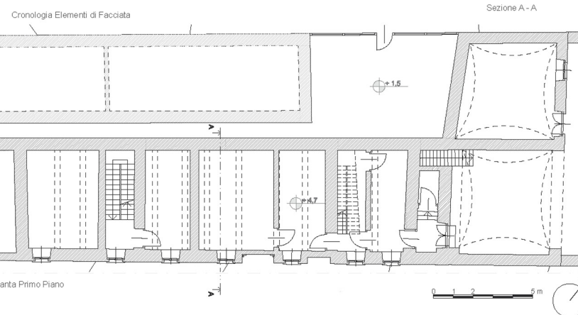
6. Architectural scale analyses of Accornero House. On the left, orthophoto and Harris Diagram, on the right, first floor plan, thematic elevation and cross section.
